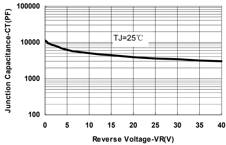
Fig.1-Typical Junction Capacitance
